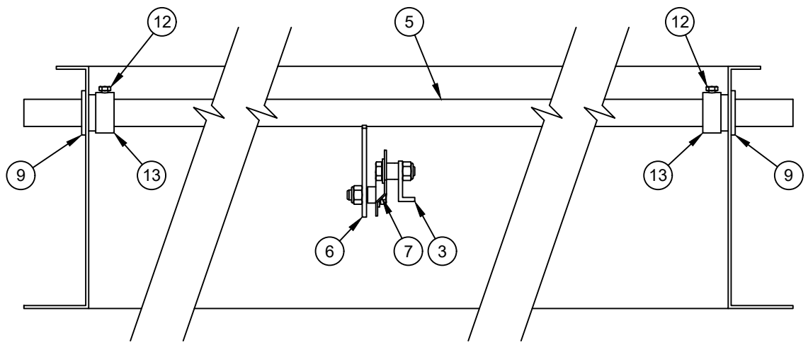
INTERNAL VIEW
