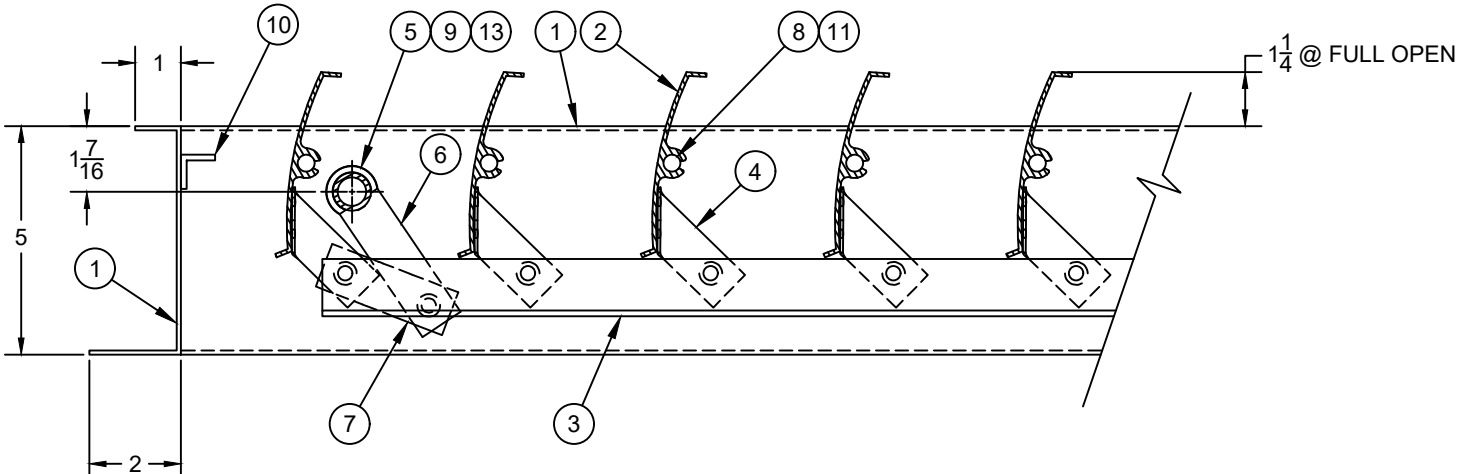
LOUVER @ FULL OPEN
