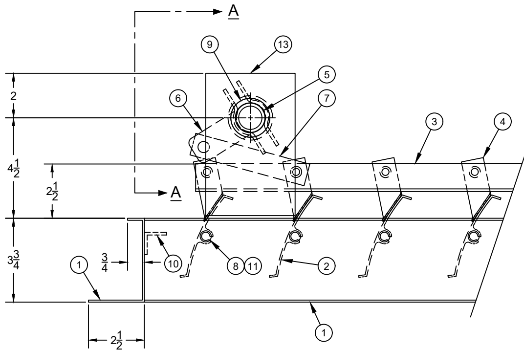
LOUVER AT FULL OPEN
