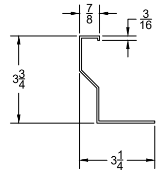
SIDEFRAME SECTION
